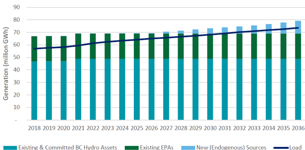
Figure 10: Cumulative Energy Generation by Existing, Committed, and New Sources by Year (2018-2036)
