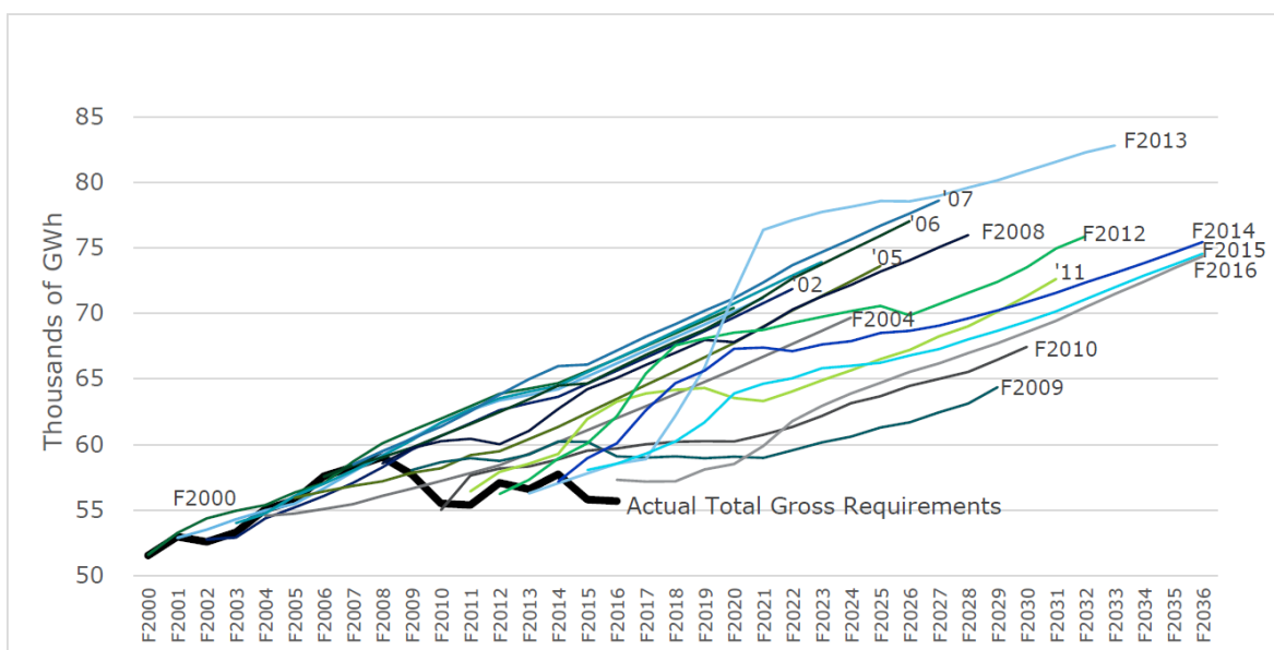
Figure 7: Total Gross Requirement Forecast Models Between 2000 and 2016(with DSM) 275
