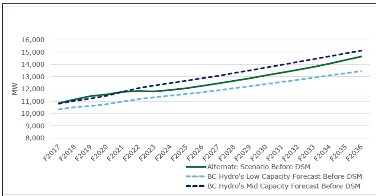
Figure 5: Capacity Forecast Before DSM - BC Hydro Mid and Low Compared with Alternate Scenario 252
