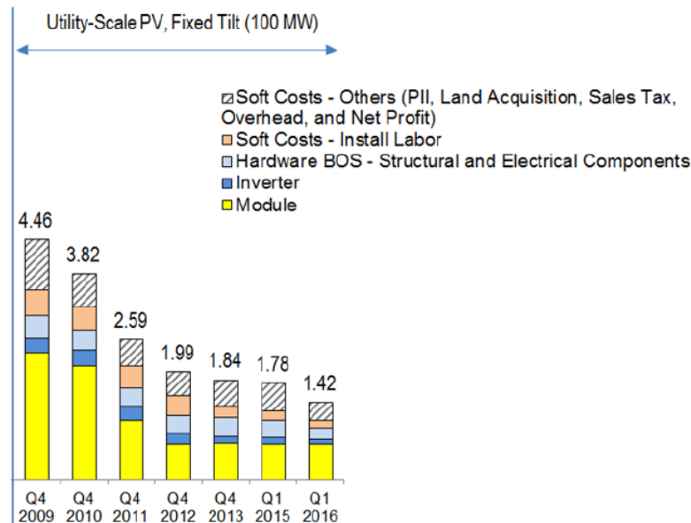
Figure 23: PV System Cost Summary (2016 USD/Watt DC)
