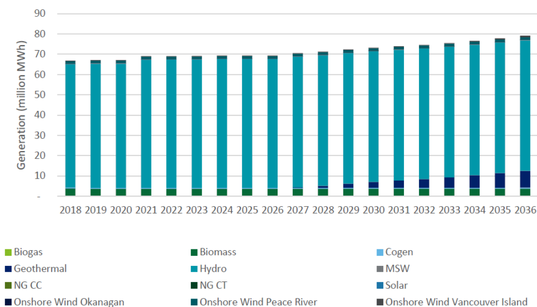
Figure 11: Cumulative Energy Generation by Resource Type by Type (2018-2036) for all resources (existing, committed and new endogenous)
