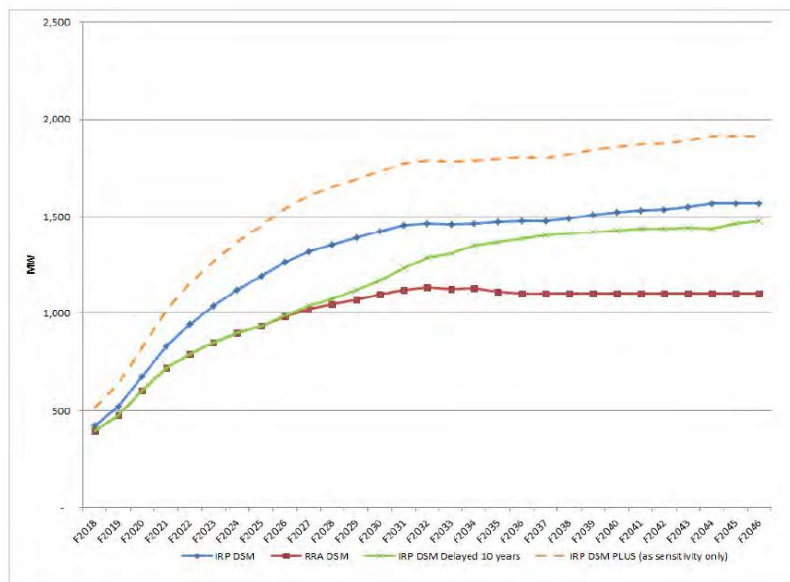
Figure 19: DSM Capacity Savings (including loss savings, mid estimate)
